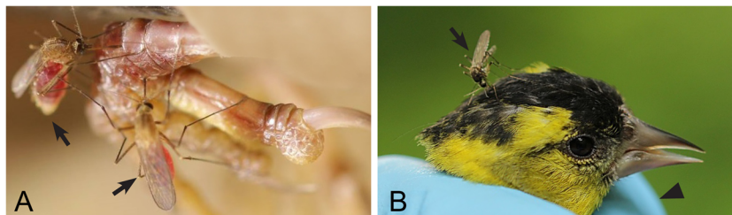
Fig. 1 Experimental exposure of Culex quinquefasciatus (a) and Ochlerotatus cantans (b) mosquitoes by allowing them to take blood meals on the legs (a) and head (b) of malaria-infected birds. Short
